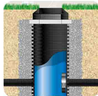
Hydro International Hydrobrake Flow Control Chamber
